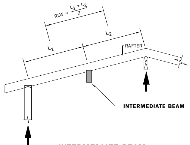
INTERMEDIATE BEAM
